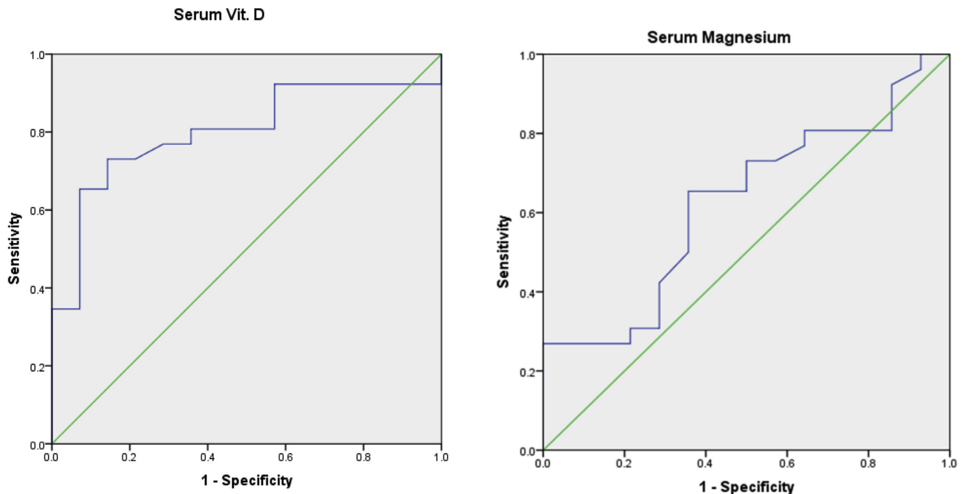
Fig. 1. Receiver operating characteristic curve(ROC) for baseline variations of Vit D and Mg+.
